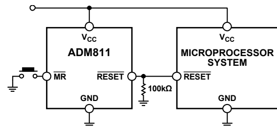
Figure 2. Typical ADM811 Operating Circuit
